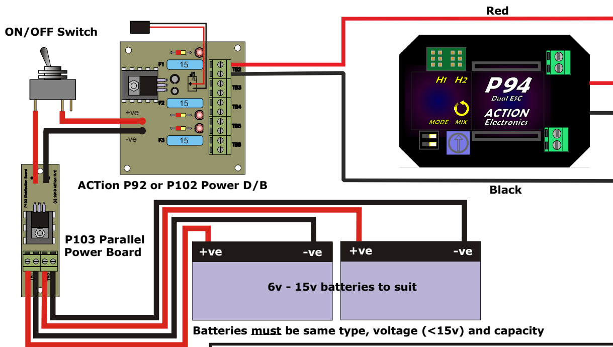
FIG #5: TWO BATTERIES CONNECTED IN PARALLEL
