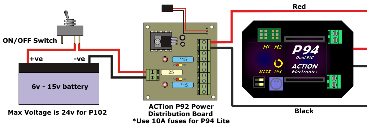
FIG #4: USING POWER DISTRIBUTION BOARD P92 OR P102
